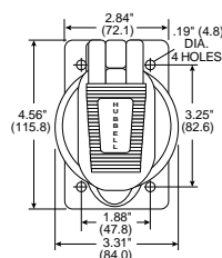
Typical Plate, Single Gang
